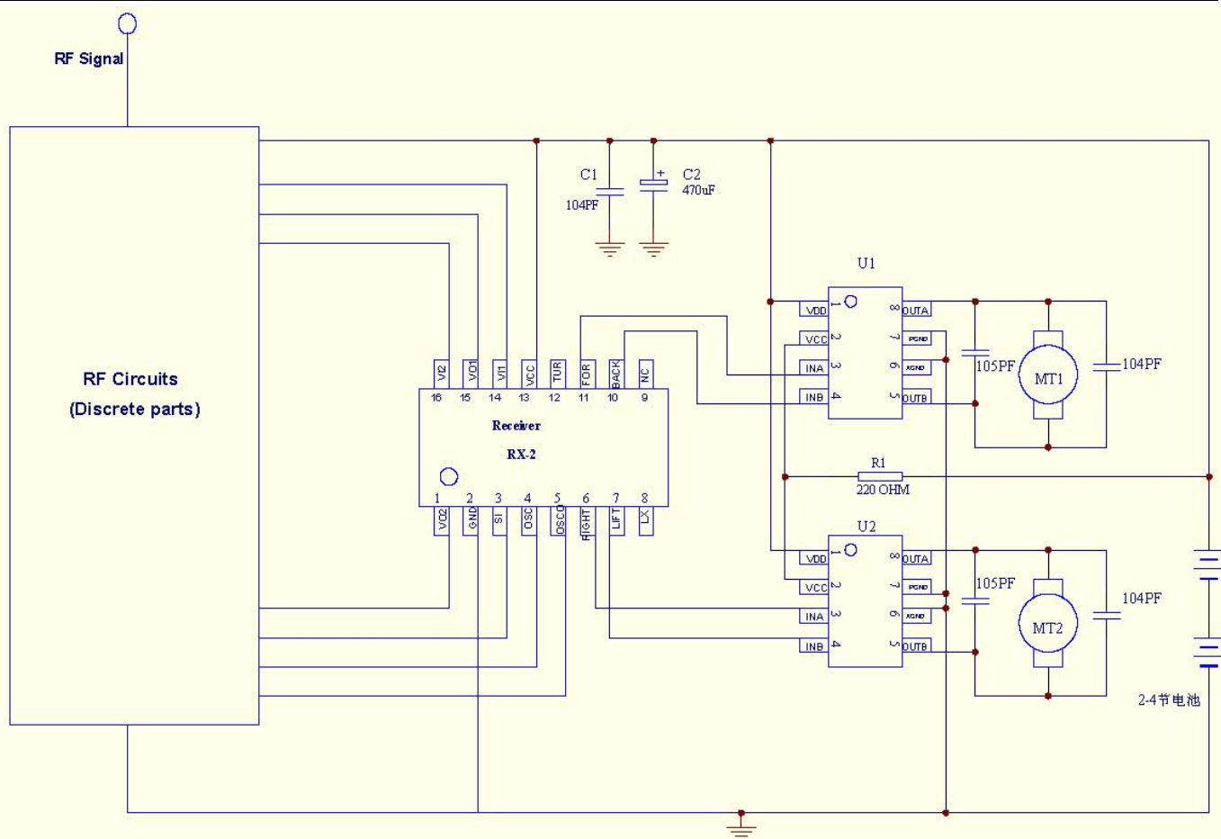
Fig.2 Schematic diagram of motor driving application circuit for 2-4 batteries operated remote control toy car
