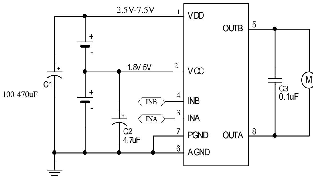
Fig.1 Schematic diagram for HG40F13 of typical application circuits
