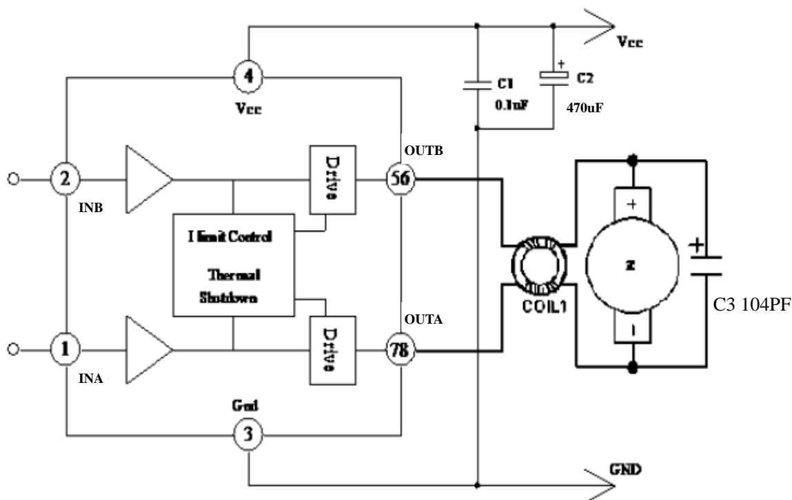
Fig.1 Schematic diagram for typical application circuits
