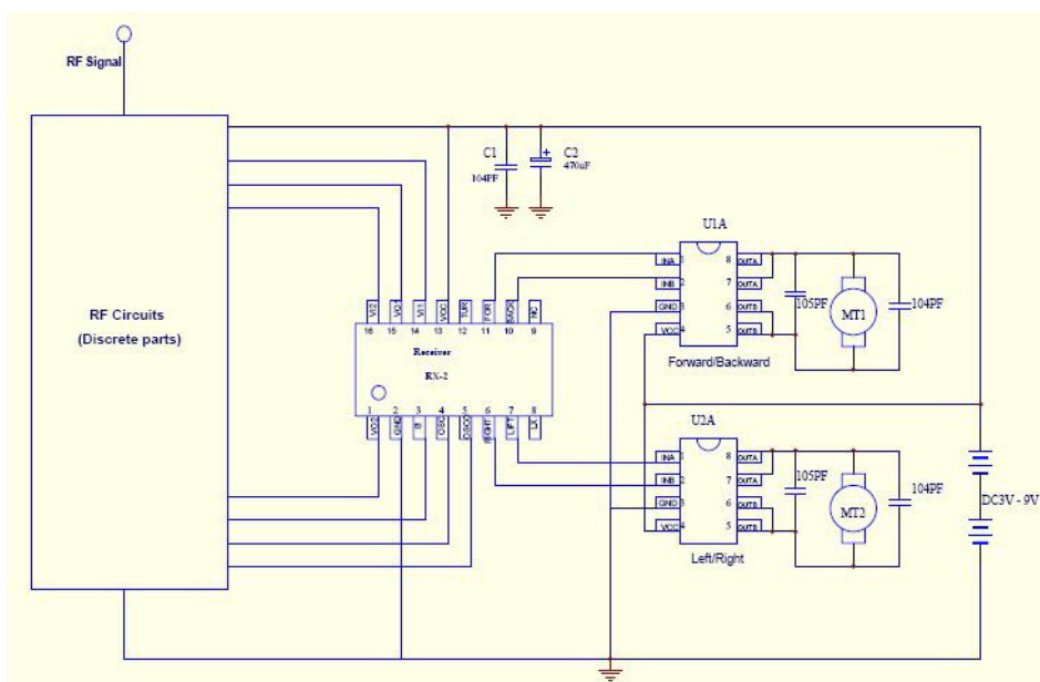
Fig.2 2-6 battery motor driver schematic diagram
