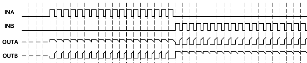
Schematic diagram of signal A waveform in PWM mode
