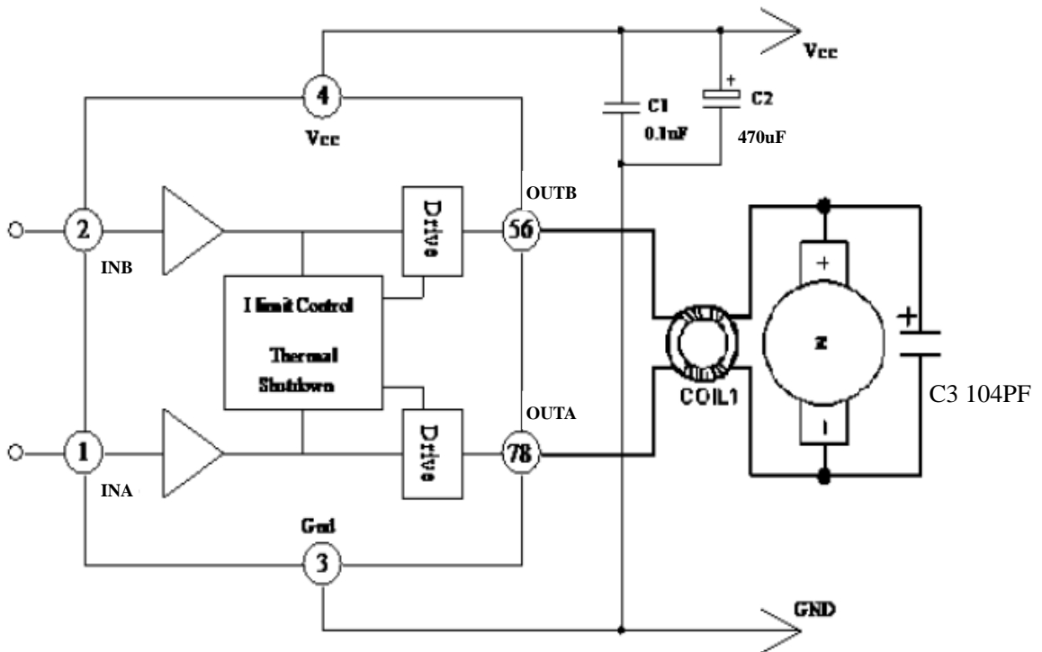
Fig.1 Schematic diagram for typical application circuits
