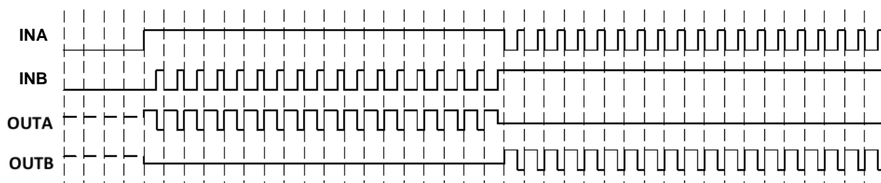
Schematic diagram of signal B waveform in PWM mode
